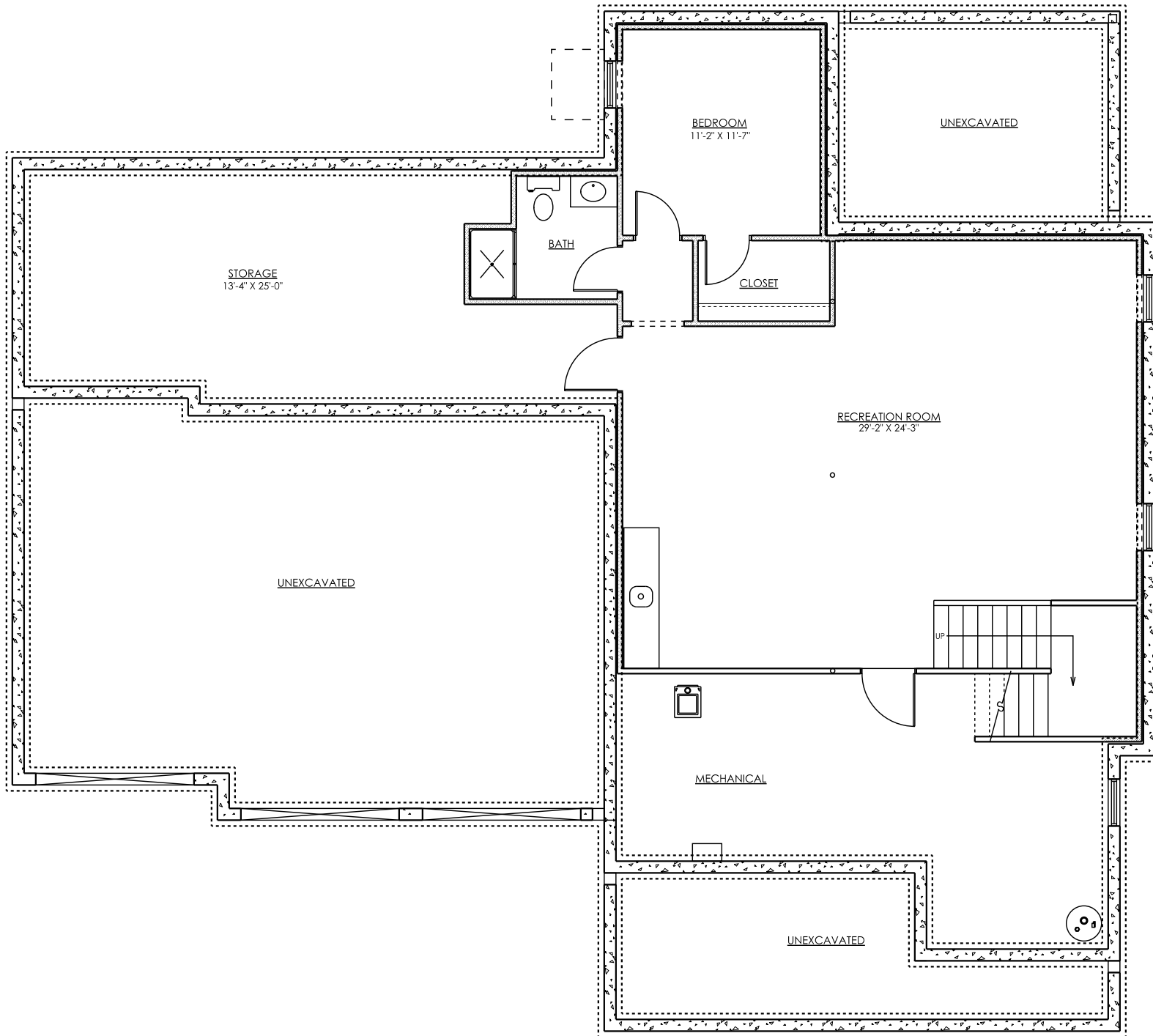
FINISHED BASEMENT PLAN
