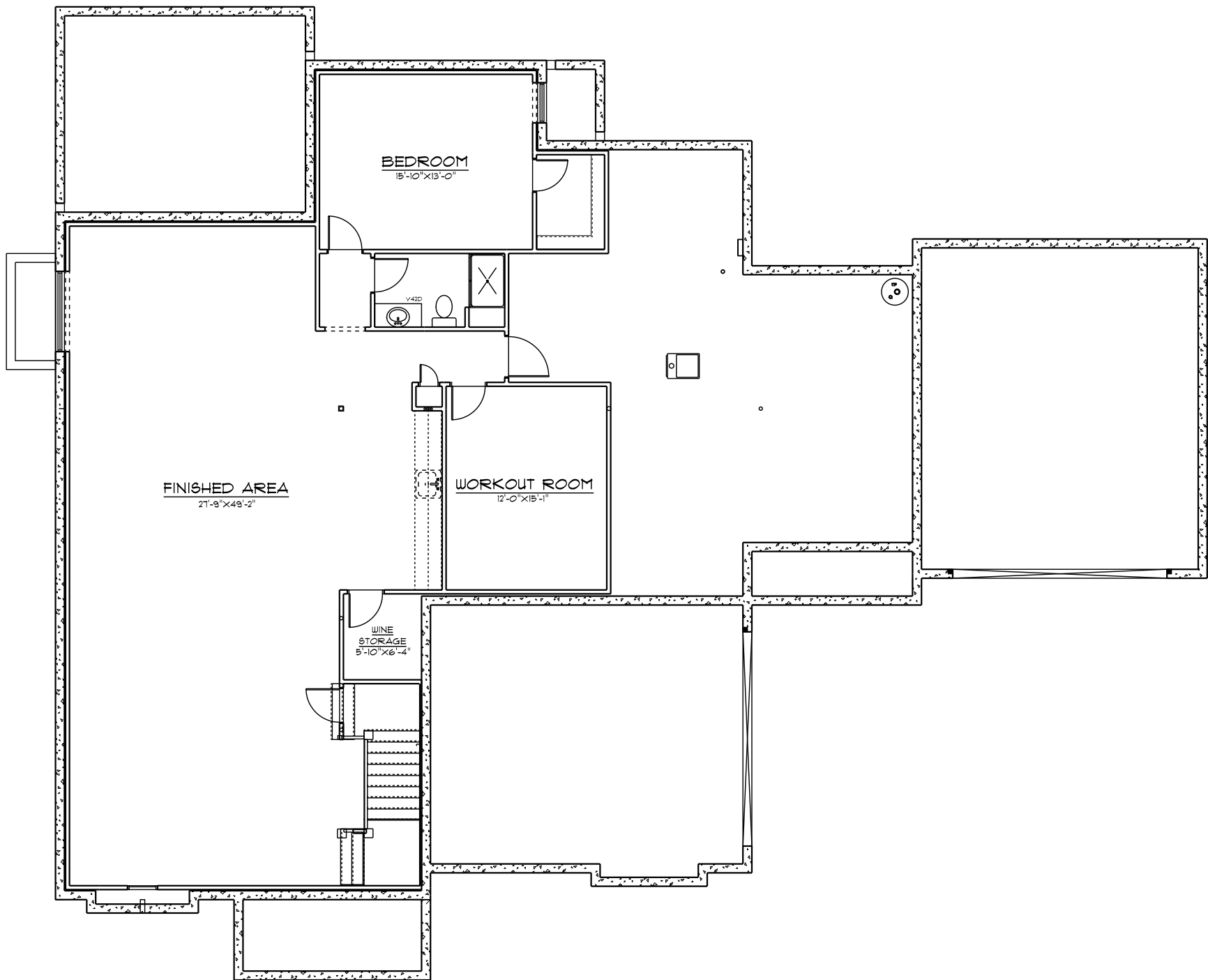
FINISHED BASEMENT PLAN
