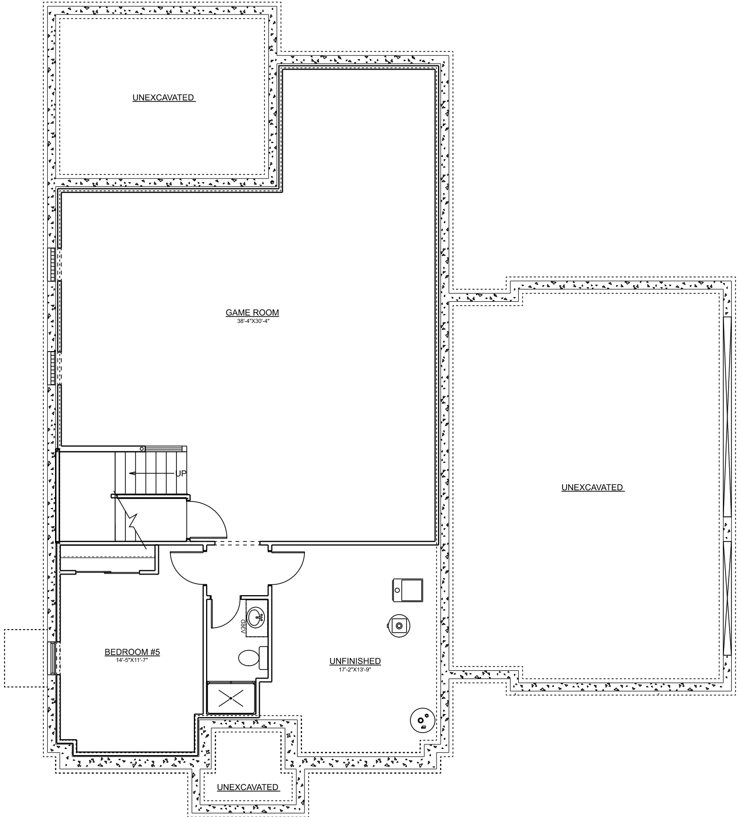
OPT. FINISHED BASEMENT PLAN
