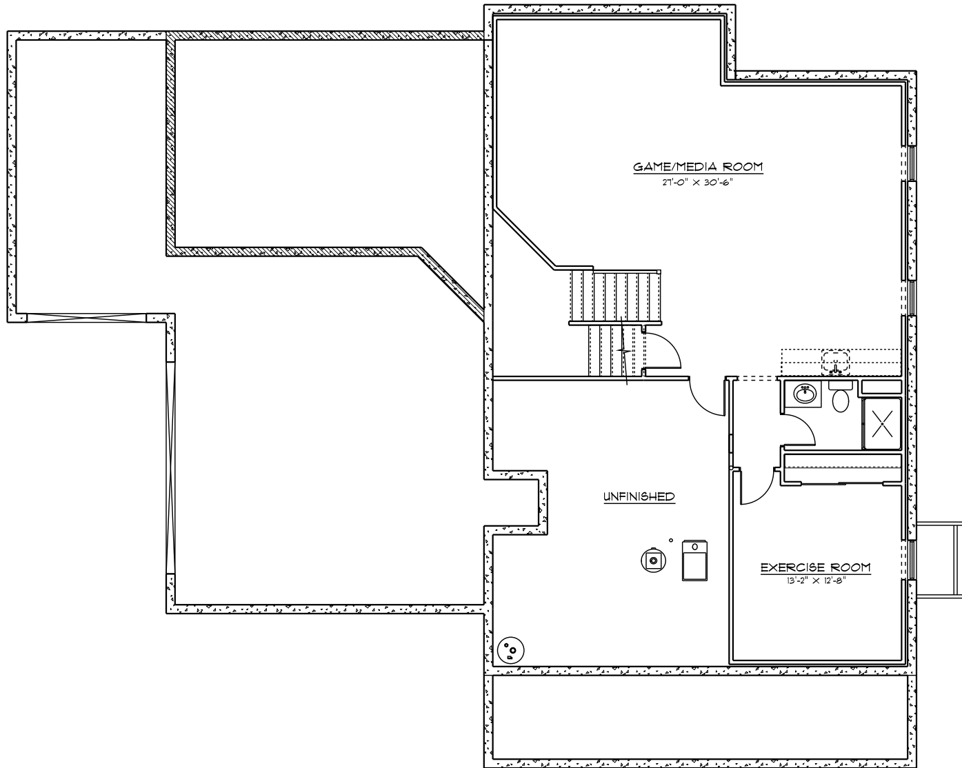
FINISHED BASEMENT PLAN
